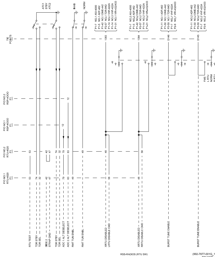
Figure 2-2. Falcon 50/50EX Retrofit Avionics System, Interconnect Wiring Diagram (Sheet 12 of 22)
