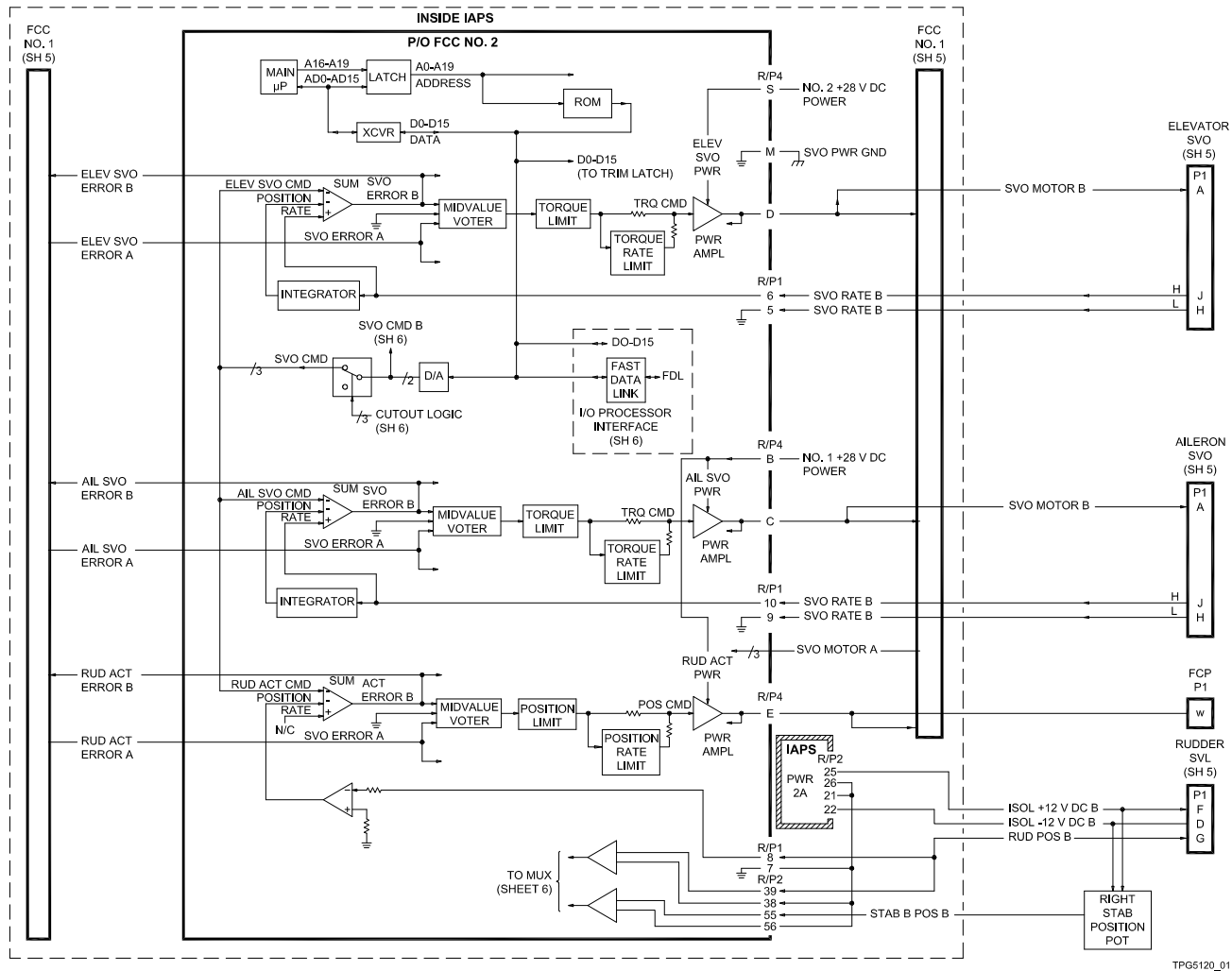
Figure 4-14. FCS System Schematic (Sheet 7 of 8)
