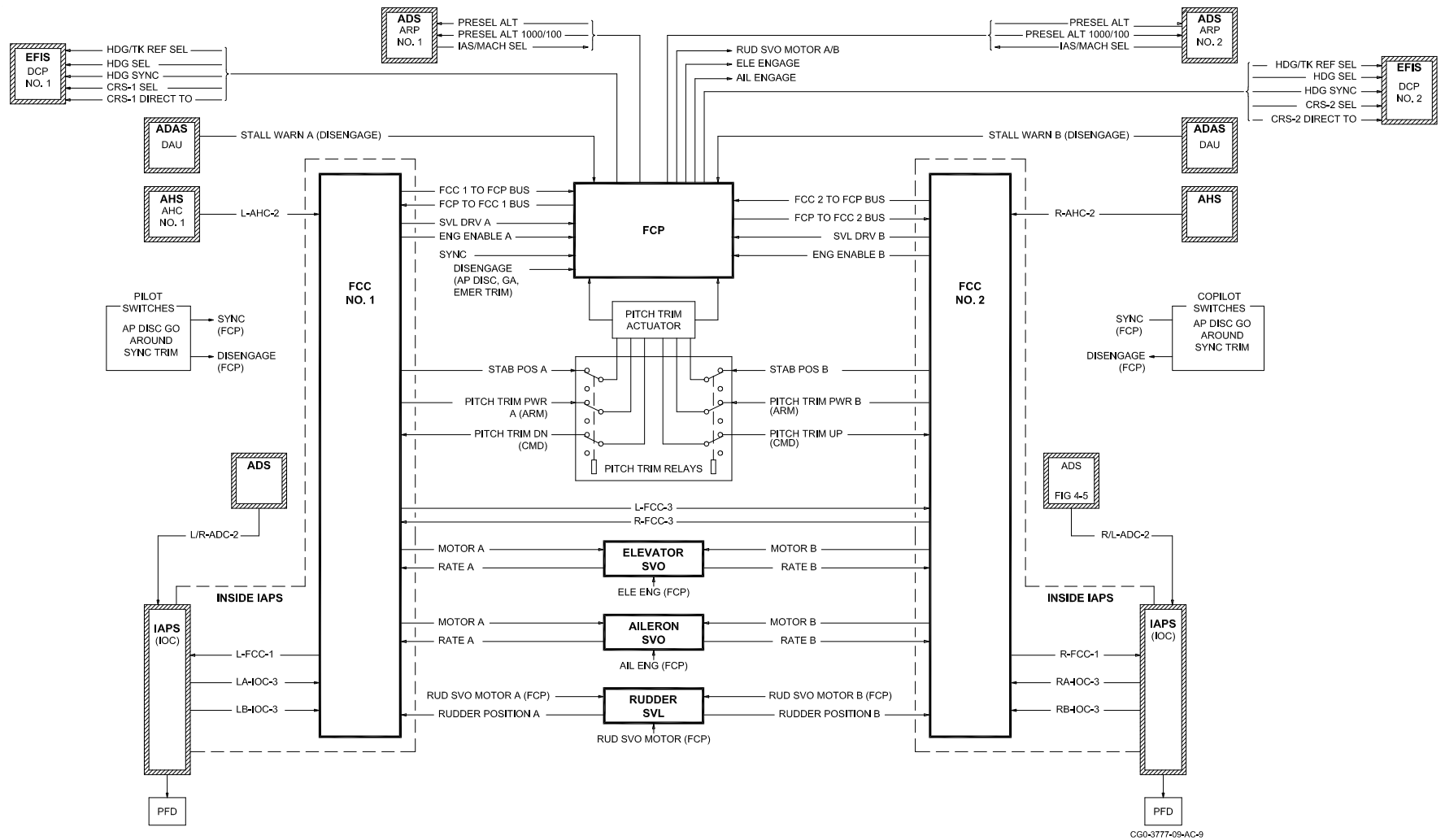
Figure 4-13. FCS (Flight Control System)
