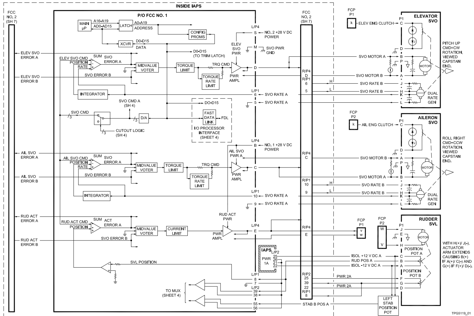
Figure 4-14. FCS System Schematic (Sheet 5 of 8)
