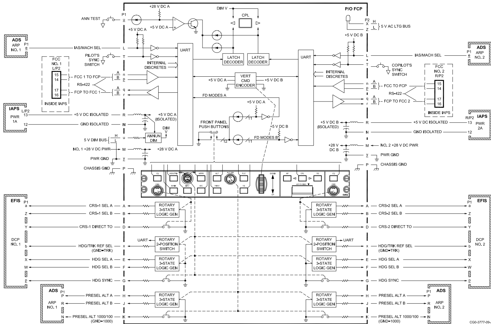
Figure 4-14. FCS System Schematic (Sheet 1 of 8)
