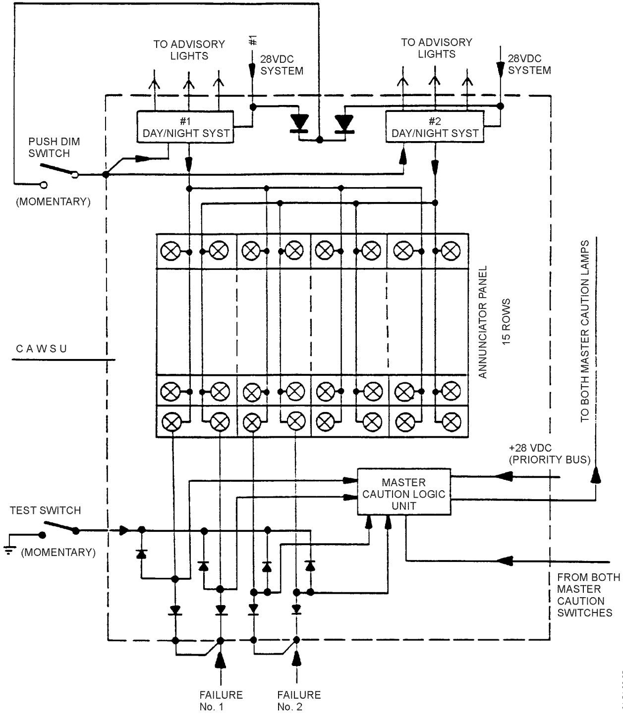
Annunciator Panel (CAWSU) - Schematic Figure 3
