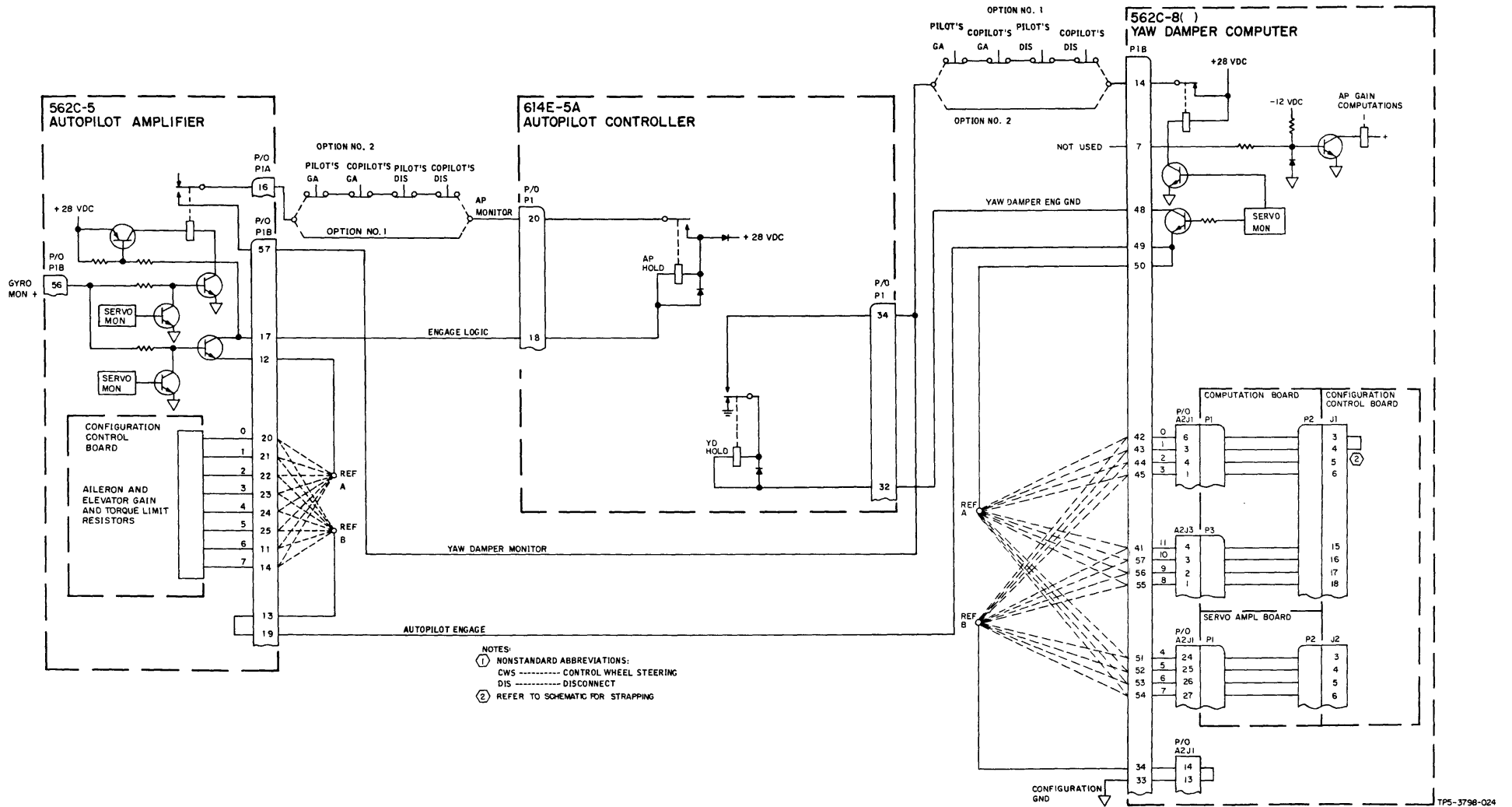
Figure 1-7. FCS-105( ) Flight Control System, Engage and Configuration Control, Interconnect Diagram
